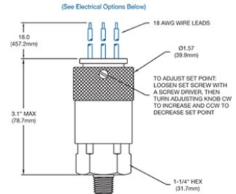
High Pressure Switch CD
