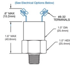
Low Pressure Switch SM
